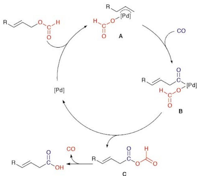
Scheme 11
