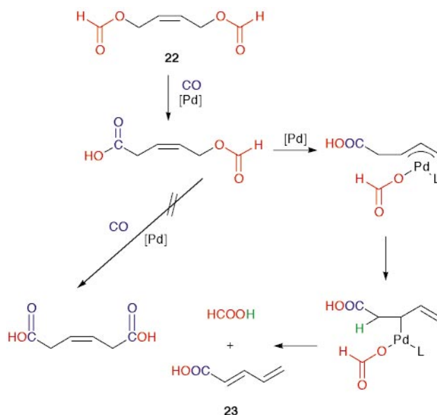
Scheme 12
